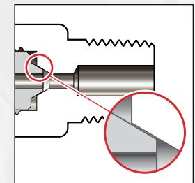
CPF to non-CPF metal seal. Use a wrench to create a seal.
